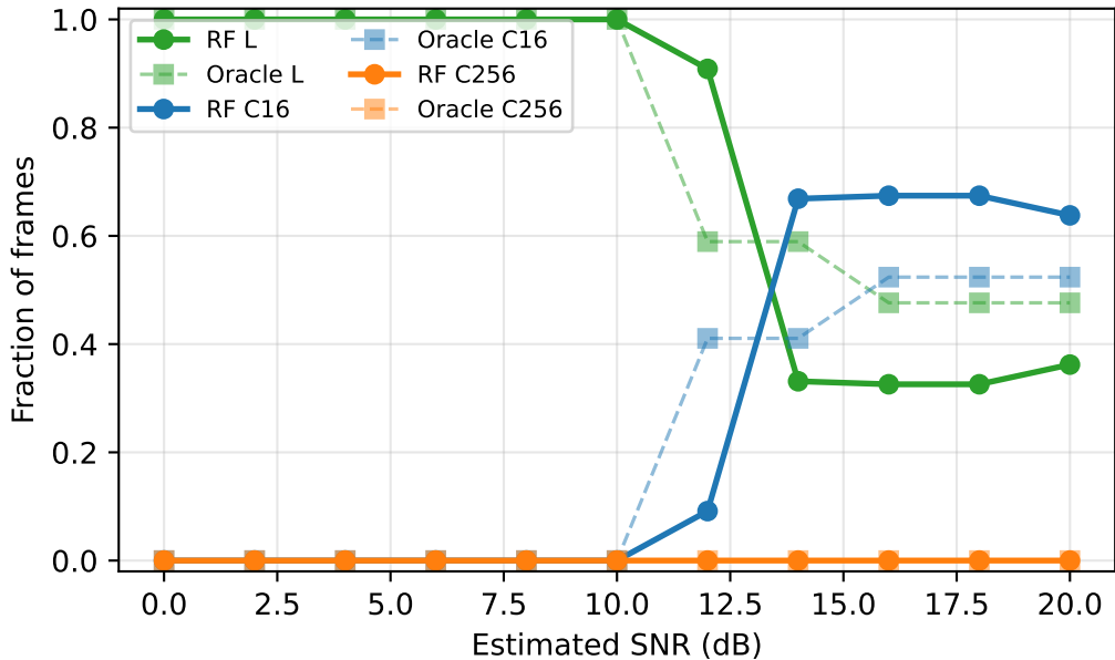
3-way selector behaviour — AWGN
