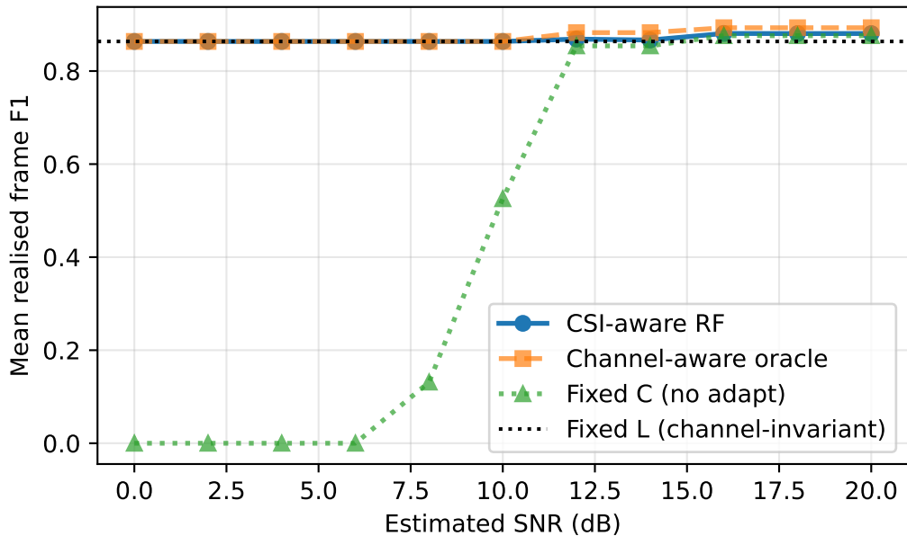
Receiver-side F1 vs channel quality
