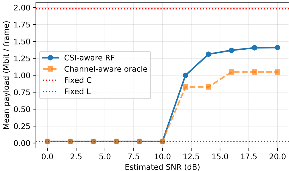
Bandwidth consumption vs channel quality
