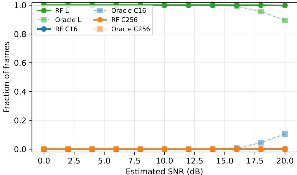
3-way selector behaviour — RAYLEIGH
