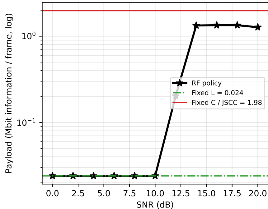
Bandwidth — AWGN
