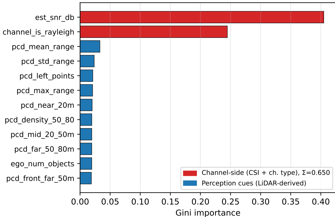
Top-12 features by Gini importance (deployed selector)
