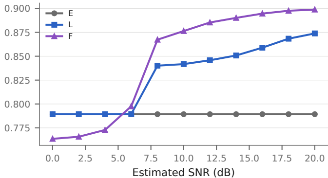
Action utility (development split)
