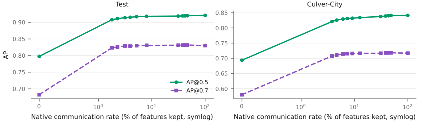
Fig. 7. Where2comm on its native communication-rate axis. The horizontal axis is the fraction of features retained, not a bit budget.
