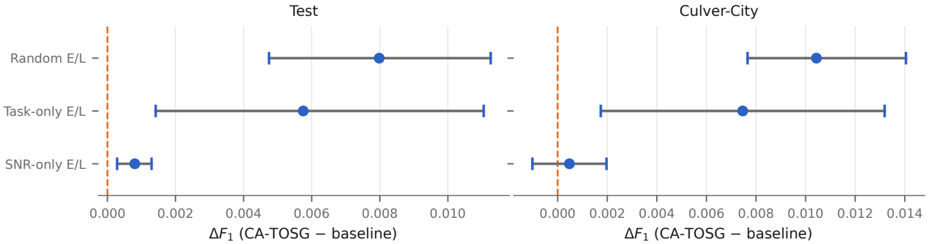
Fig. 4. The same differences as Table VI, drawn: \Delta F_1 between CA-TOSG and each deployable baseline at matched realised payload, with 95% scene-level bootstrap intervals and a dashed line at zero. Secondary analysis, not preregistered. Payload is matched numerically to within 2.3 \times 10^{-7} Msym, not exactly. Culver-City carries 4 scenes, so its intervals are coarse—visibly so against the SNR-only rule, whose interval crosses zero. The non-deployable greedy references are not shown.
