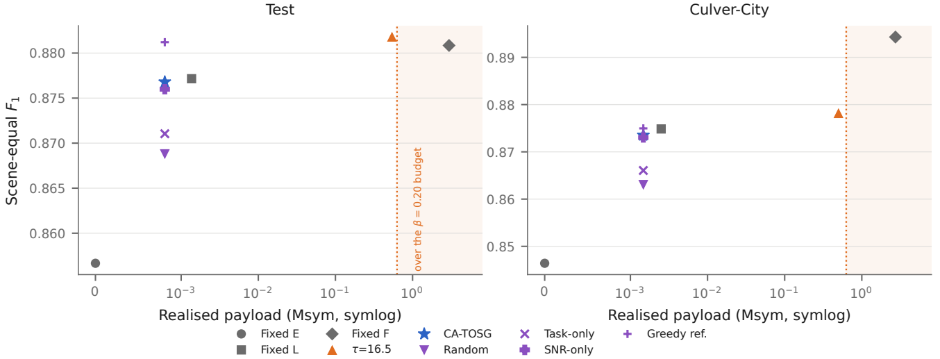
Fig. 3. Scene-equal F_1 against realised payload on each held-out split. Both quantities are shown together, because ranking on either alone misrepresents the trade-off: the arms differ by more than three orders of magnitude in payload—at least 1,090\times between Fixed L and Fixed F on either split—and by hundredths in F_1 . The dotted line is the \beta = 0.20 ceiling and the shaded region is over budget, so Fixed F is visibly not a competitor at the primary budget. The x axis is symlog rather than logarithmic: Fixed E spends exactly zero, which a logarithmic axis cannot show. Random, Task-only, SNR-only and the greedy reference are the matched-payload policies of Table VI and sit at CA-TOSG’s own payload. The plotted reference is the gain-per-cost one of the two in Table VI; it is not deployable and is not a proven optimum.
