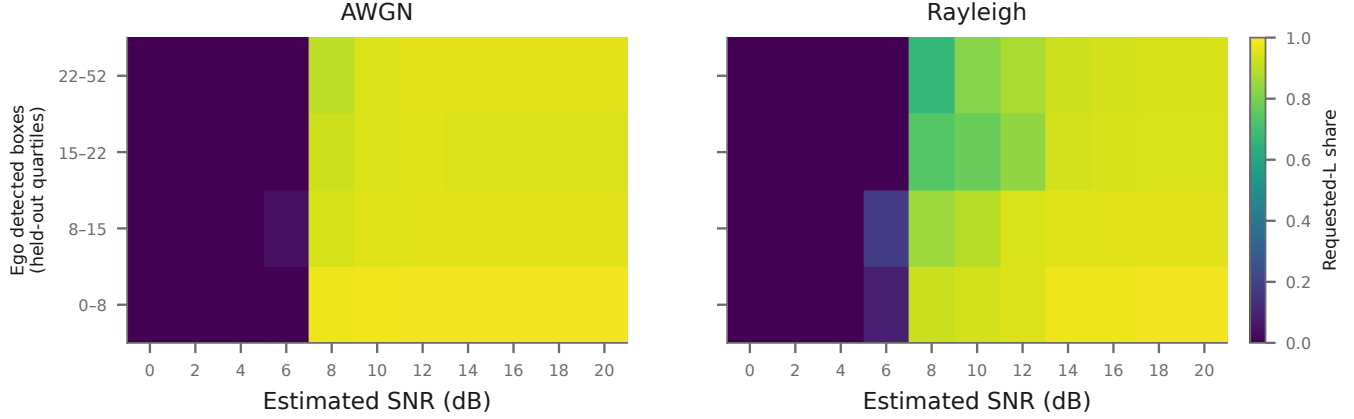
Fig. 5. Where the frozen policy requests object-level cooperation, pooled over both held-out splits. Colour is the requested-action share of L; frames without an available collaborator are structurally executed as E and are counted here by what was requested, never by what was executed. The horizontal axis is the 11 protocol SNR grid points and the vertical axis is the ego detected box count in quartiles of the pooled held-out rows, both fixed before plotting; cells are drawn without smoothing or interpolation, so no structure is shown between points that were evaluated.
