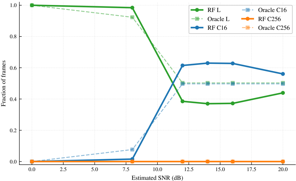
3-way selector behaviour — AWGN
