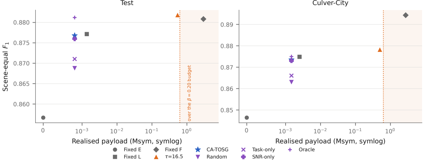
Fig. 2. Scene-equal F_1 against realised payload on each held-out split. Both quantities are shown together, because ranking on either alone misrepresents the trade-off: the arms differ by up to 1,244\times in payload and by hundredths in F_1 . The dotted line is the \beta = 0.20 ceiling and the shaded region is over budget, so Fixed F is visibly not a competitor at the primary budget. The x axis is symlog rather than logarithmic: Fixed E spends exactly zero, which a logarithmic axis cannot show. Random, Task-only, SNR-only and Oracle are the matched-payload policies of Table IV and sit at CA-TOSG's own payload; Oracle is not deployable.
