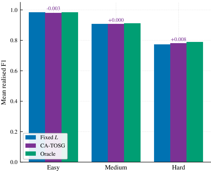
OPV2V test: all channels
