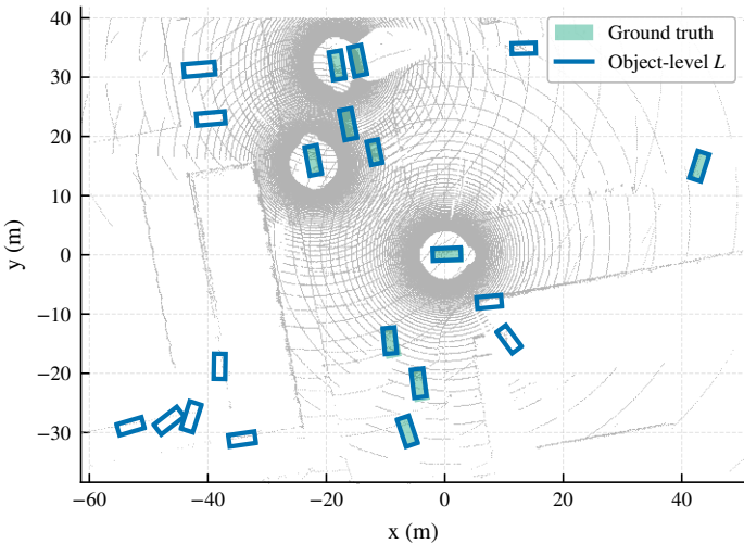
Object-level L (F1 = 0.67)
