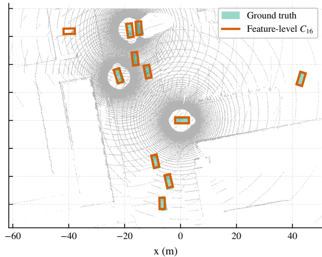
Feature-level C_{16} (F1 = 0.95)
