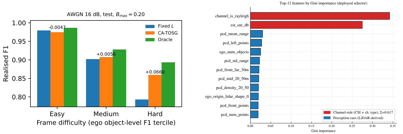
Fig. 6. Left: realised F1 by frame-difficulty tercile (ego object-level F1) on OPV2V test at B_{\max} = 0.20 at a single reliable-channel grid point (AWGN 16 dB) with the frozen selector; numbers above bars are CA-TOSG—Fixed- L , the hard-frame gain being +0.0660 (95% CI [+0.0591, +0.0730]). Right: top-12 features by Gini importance of the frozen B_{\max} = 0.20 selector—the channel-side features jointly account for 61.7%, the 21 perception-side cues for the remaining 38.3%, none above 3.0% alone. Importance is not sufficiency (Section VI-C).
