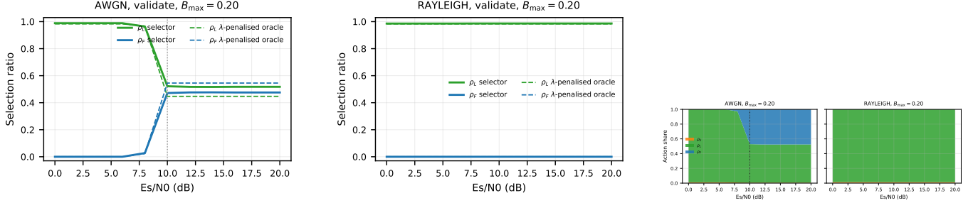
Fig. 5. Per-mode selection ratios versus SNR on OPV2V validate at B_{\max} = 0.20 , from the frozen grid. Top: the frozen selector (solid) against that budget’s \lambda -penalised oracle (dashed) — the oracle sees the frame BLER, not the per-frame block outcome, so it is not clairvoyant. Bottom: stacked-area view of the selector’s action distribution over the deployed action set S = \{E, L, F\} under AWGN and Rayleigh (the dominated C_{256} is a physical-layer comparator, not a deployed action, Section III-B); the dotted line marks the measured 10 dB policy knee. Two readings: under AWGN \rho_F steps from 0 to 0.472 at 10 dB and is flat above it, and under Rayleigh the selector’s \rho_E is 0.002 (test) / 0.000 (Culver-City) while the oracle spends \rho_E = 0.157 / 0.133 there — the E -collapse limitation of Section ?? . The three-budget version is Fig. ??.
