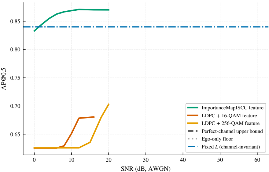
Feature-branch coding: JSCC (graceful) vs LDPC (cliff)
