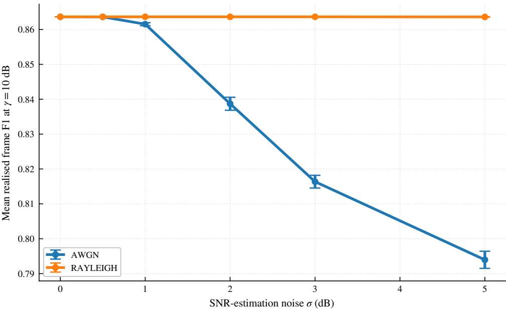
CSI-noise robustness of the deployed selector
