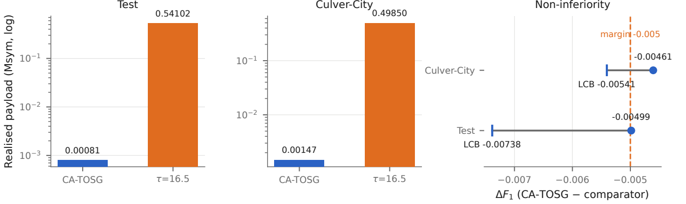
Fig. 2. Primary cell. Payload is drawn on a logarithmic axis and \Delta F_1 in its own panel: the two halves of the result differ by three orders of magnitude, and a shared scale would erase one of them. The right panel puts the preregistered margin and the bootstrap lower bound on one ruler. On both splits the point estimate lies inside the margin and the bound does not.
