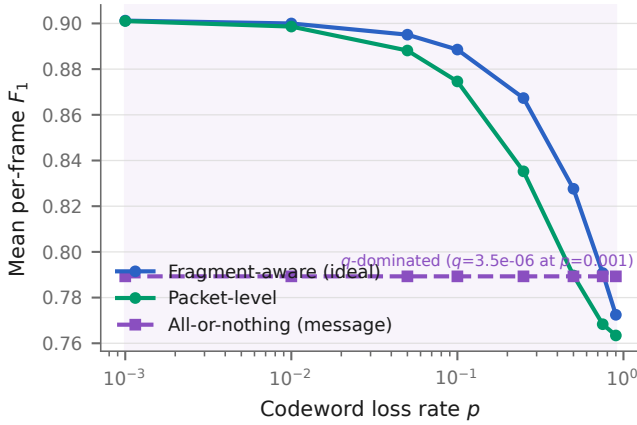
Fig. 3. Delivery regimes on the development split. Fragment-aware partial recovery degrades gracefully; all-or-nothing message delivery is governed by the survival probability q rather than by how the feature action performs.
