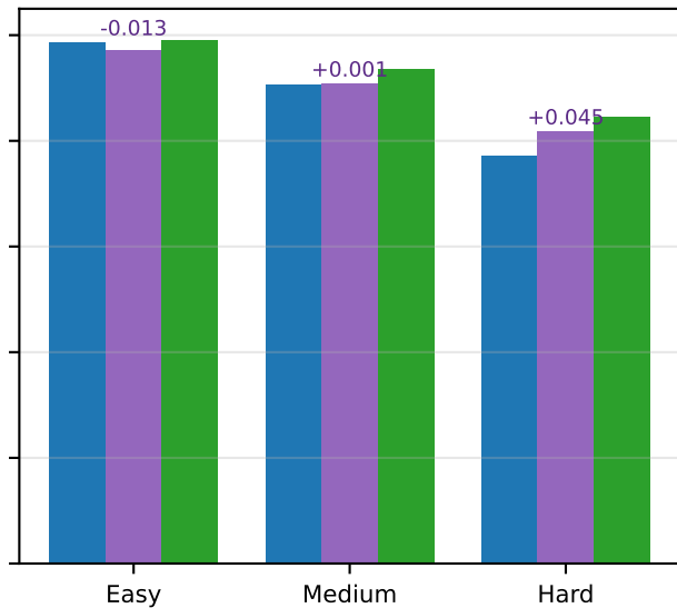
OPV2V test: AWGN, SNR \geq 14 dB
