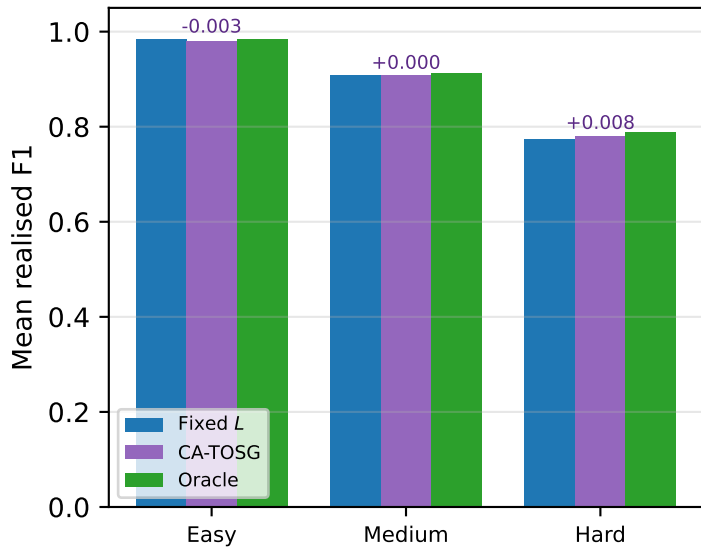
OPV2V test: all channels
