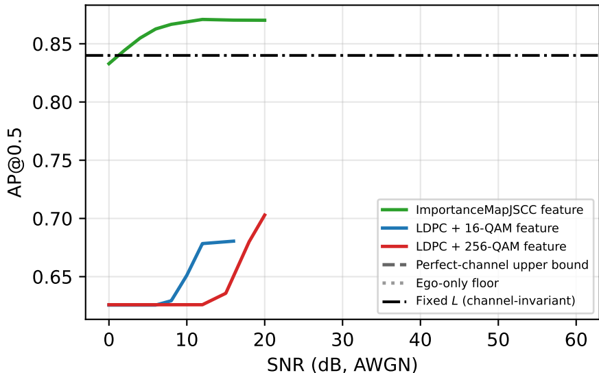
Feature-branch coding: JSCC (graceful) vs LDPC (cliff)
