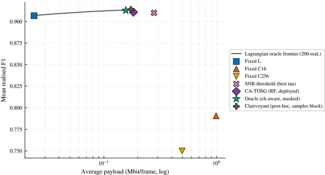
OPV2V validate (200 channel realisations)
