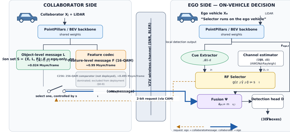
Fig. 1. Overview of the proposed CA-TOSG framework. The ego vehicle extracts online task cues z_t and estimated channel quality (\gamma_t, ch_t) , then selects one communication mode s_t \in S = \{E, L, F\} , where E is ego-only operation with no request at all (the dominated C_{256} mode is a physical-layer comparator and is not in the deployed action set, Section III-B). Only the selected message is transmitted through the V2V link and fused with the local ego feature F_{ego,t} for 3D object detection.
