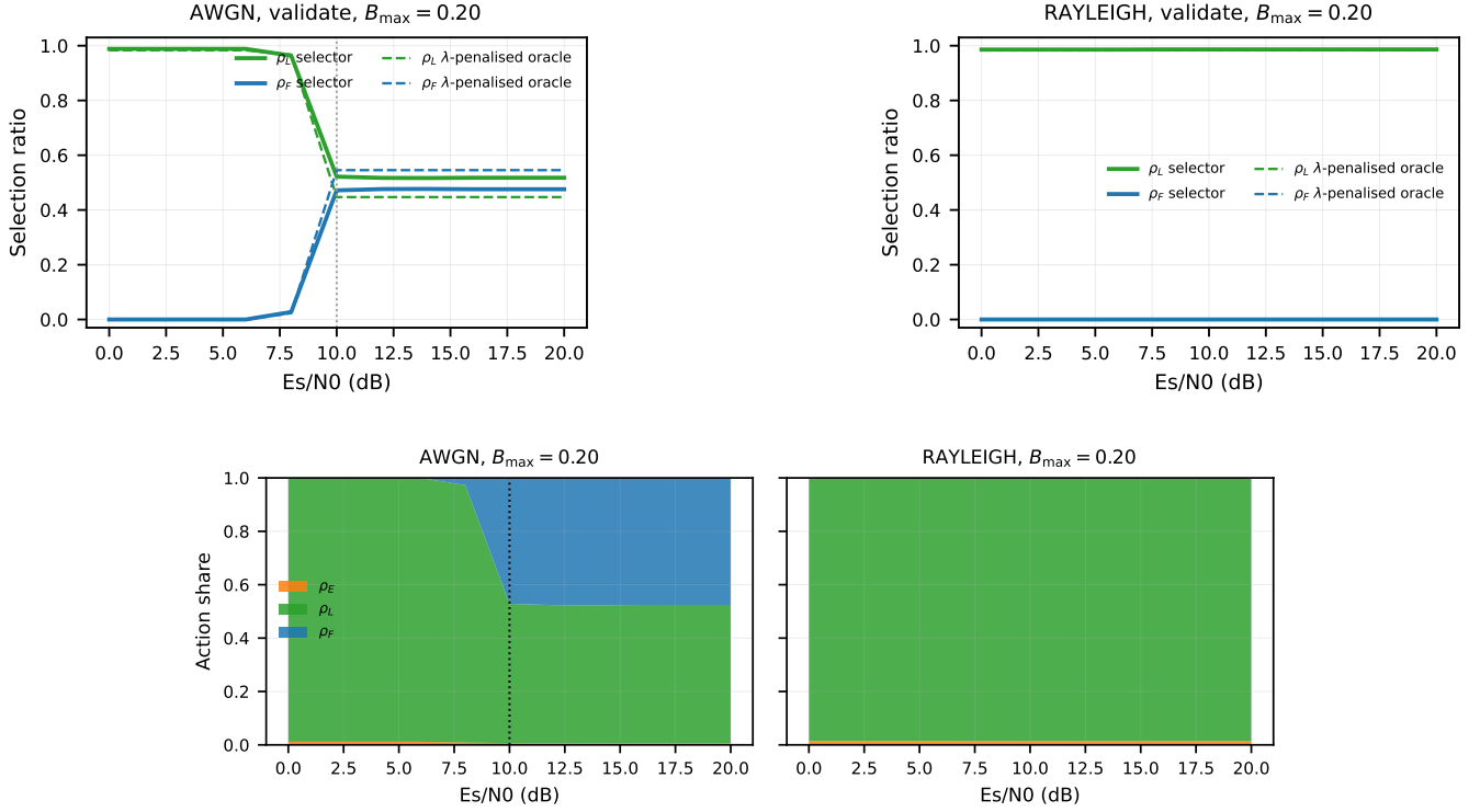
Fig. 4. Per-mode selection ratios versus SNR on OPV2V validate at B_{\max} = 0.20 , from the frozen grid. Top: the frozen selector (solid) against that budget's \lambda -penalised oracle (dashed) — the oracle sees the frame BLER, not the per-frame block outcome, so it is not clairvoyant. Bottom: stacked-area view of the selector's action distribution over the deployed action set \mathcal{S} = \{E, L, F\} under AWGN and Rayleigh (the dominated C_{256} is a physical-layer comparator, not a deployed action, Section III-B); the dotted line marks the measured 10 dB policy knee. Two readings: under AWGN \rho_F steps from 0 to 0.472 at 10 dB and is flat above it, and under Rayleigh the selector's \rho_E is 0.002 (test) / 0.000 (Culver-City) while the oracle spends \rho_E = 0.157 / 0.133 there — the E -collapse limitation of Section VI-G. The three-budget version is the per-budget action distributions (repository figure product).
