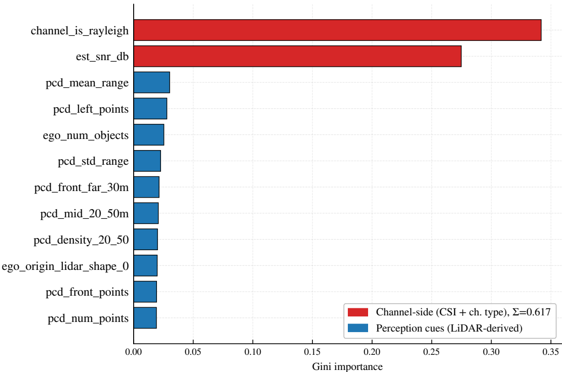
Top-12 features by Gini importance (deployed selector)
