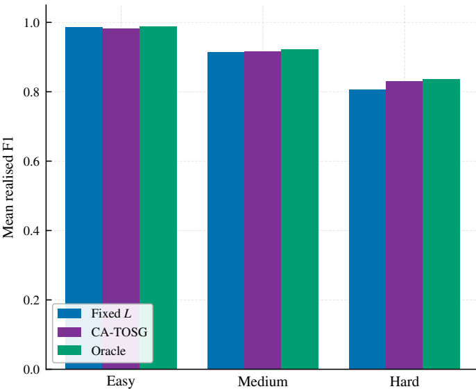
OPV2V test: all channels (200 real.)
