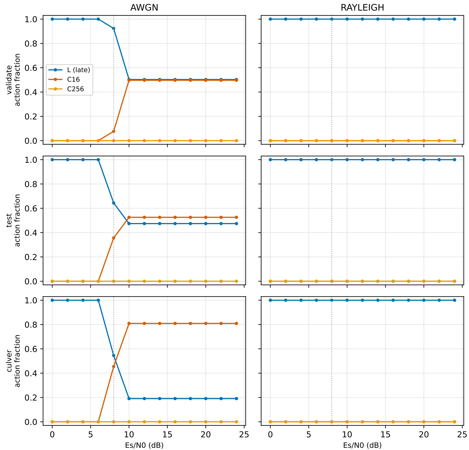
Feasibility-masked oracle action distribution vs SNR (dotted = 8 dB AWGN cliff)
