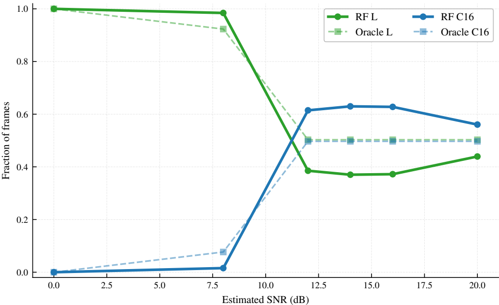
Selector vs oracle action share — AWGN
