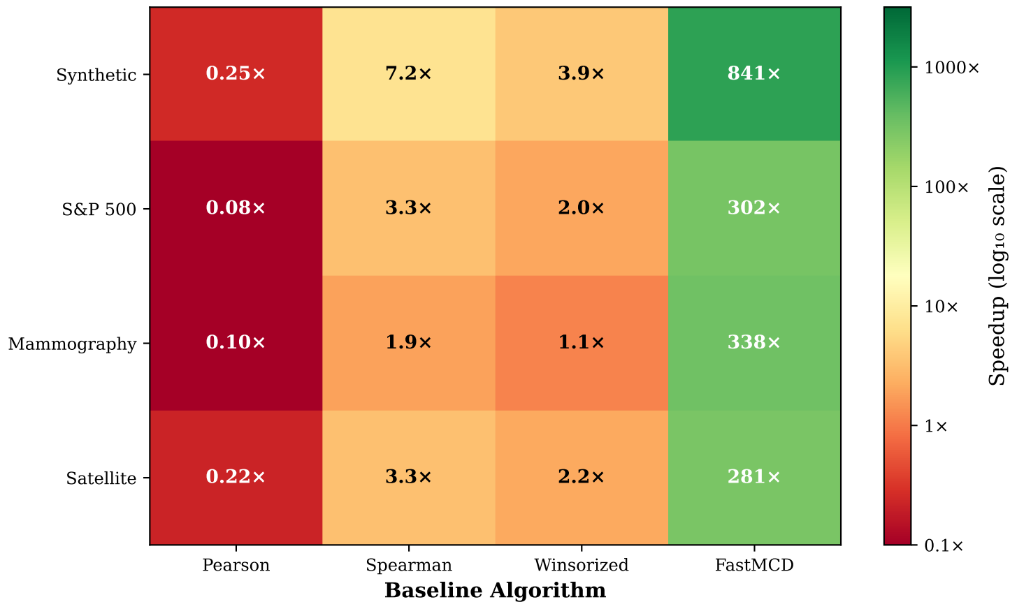
FORCE Speedup Over Baseline Algorithms
