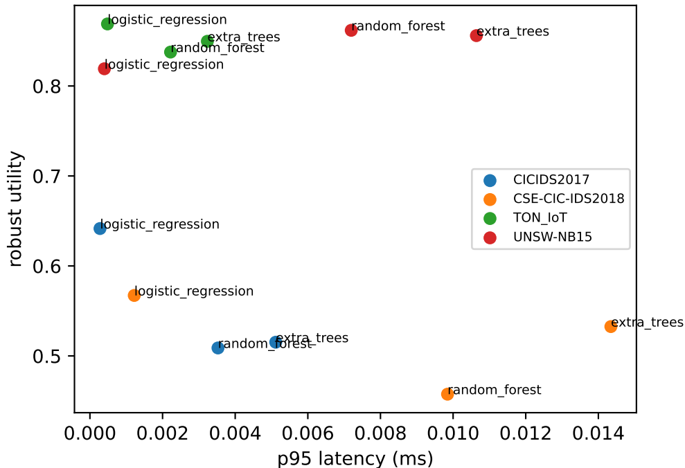
Constrained-attack robust utility vs. p95 latency
