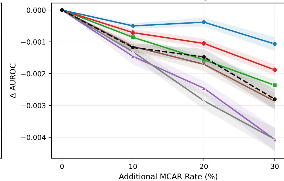
Bank Marketing
