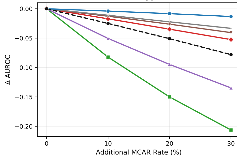
Covertype
