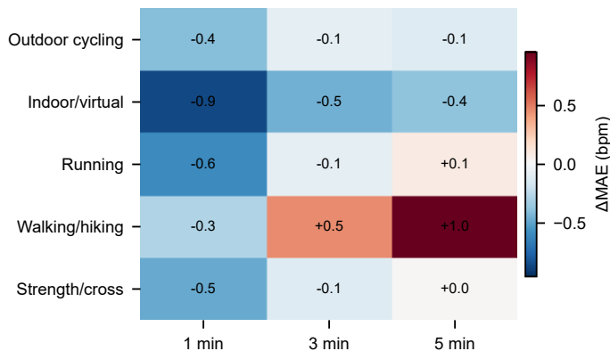
c Median model – deterministic EWMA
