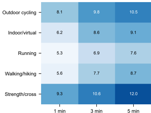
c Median model – deterministic EWMA
