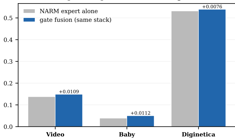
(b) Expert swap: fusion over strong NARM
