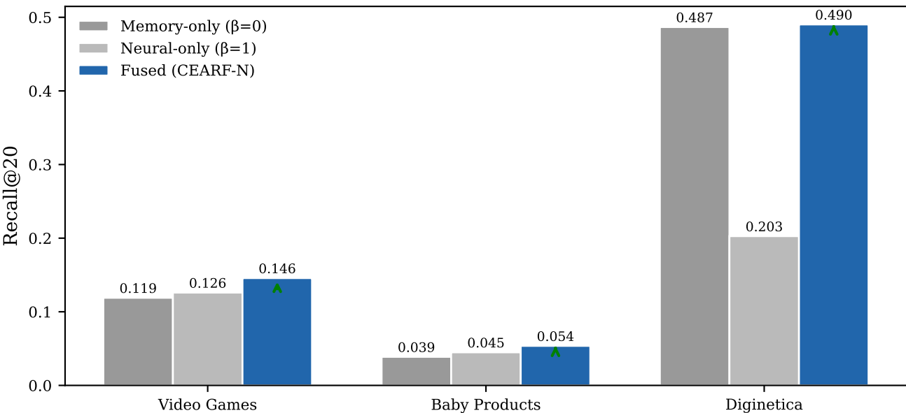
Fusion ablation: memory-only vs neural-only vs fused
