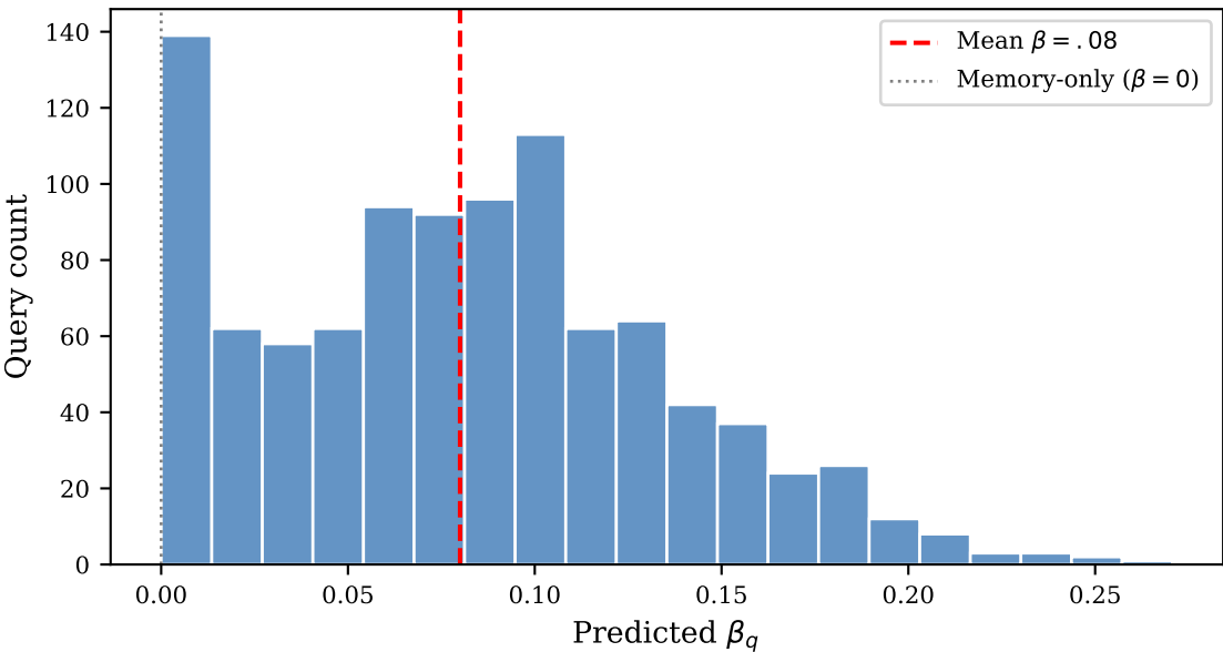
Diginetica: \beta Concentrated Near Zero, Yet +.042 R@20 Gain
