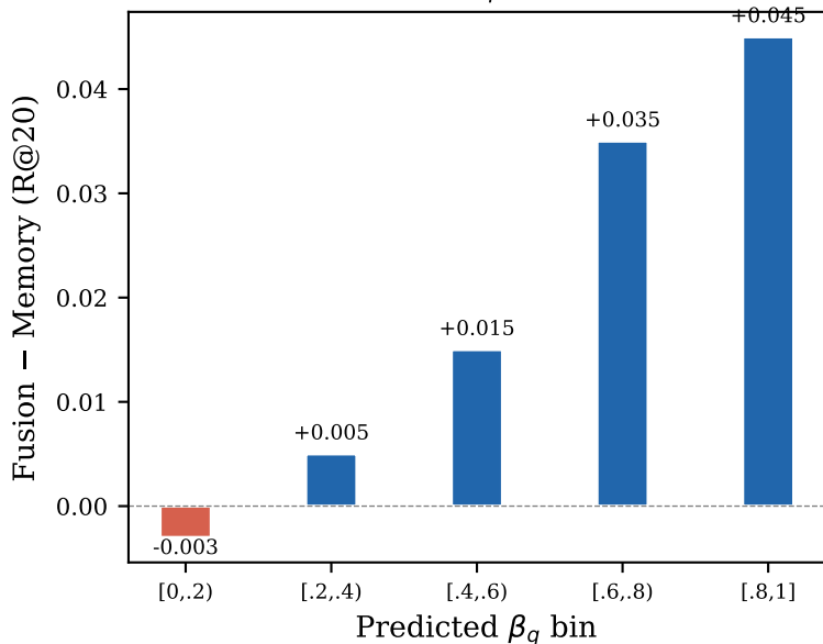
Fusion Gain by \beta_q (Video Games)
