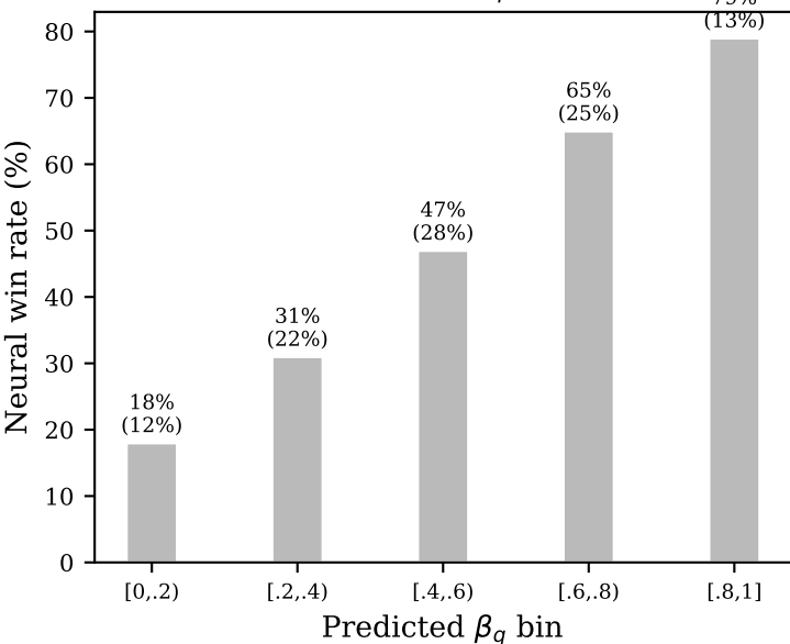
Neural Win Rate by \beta_q (Video Games)
