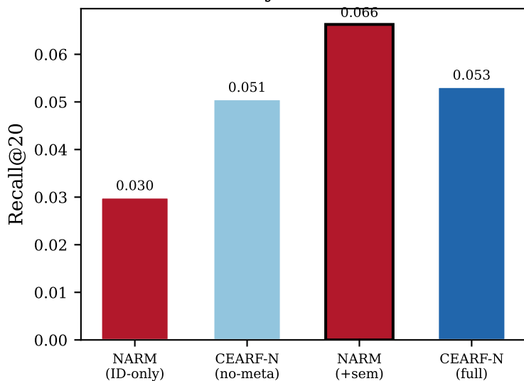
Baby Products
