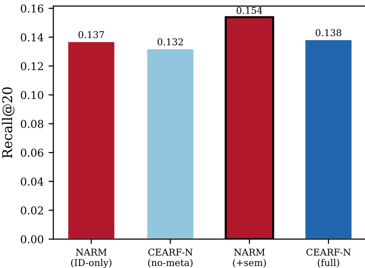
Video Games
