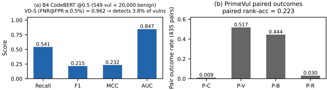
Figure 5: B4 CodeBERT baseline. (a) Threshold-0.5 metrics on the realistic arm (549 vulnerable + 20,000 benign test-split functions); VD-S is reported as the FNR at the \text{FPR} \leq 0.5\% operating point (lower is better: \approx 3.8\% of vulnerable functions detected under the budget). (b) PrimeVul paired outcomes over 435 pairs. Source: outputs/transformer/codebert_eval_vd_s_metrics.json.
