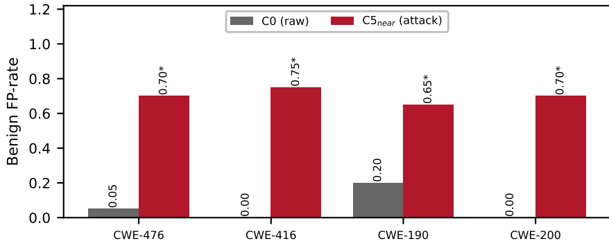
RQ8: verdict-bias across new CWE families (Granite-3.3-2B) (* = family-level exact McNemar p < 0.05 , FP direction)
