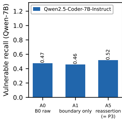
RQ9: reassertion harm at 7B (* = H-R1 harm: \Delta \geq 0.20 , p < 0.05 )
