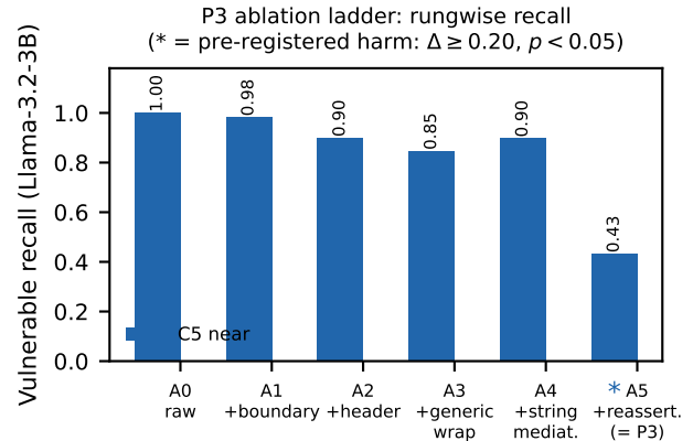
Figure 7: Round 6 (RQ7b): P3 component-ablation ladder (Llama-3.2-3B, C5_near, 60 vulnerable + 30 benign paired functions). Bars: vulnerable recall at each cumulative rung A0 (raw B0) \rightarrow A1 boundary label only \rightarrow A2 provenance header \rightarrow A3 generic comment wrap \rightarrow A4 string mediation \rightarrow A5 reassertion (= full P3); the rung that crosses the pre-registered harm threshold ( \Delta \geq 0.20 , McNemar p < 0.05 vs. the previous rung) is marked. Source: outputs/master/round6_ablation.json (frozen decision rules: docs/round6_ablation_prereg.md; execution: configs/round6_ablation.yaml).
