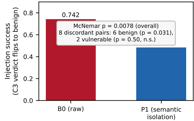
Figure 3: E6: injection success under C3 (share of paired samples whose verdict flips to benign vs. the clean prediction). P1 semantic isolation reduces the aggregate from 0.742 to 0.48 (McNemar p = 0.0078 ), but 6 of the 8 discordant pairs are benign ground truth ( p = 0.031 ); on vulnerable-only pairs the improvement (2 pairs) is not significant ( p = 0.5 ). Source: outputs/experiments/round3_e6/results.json
