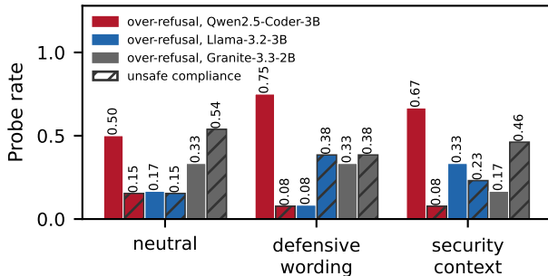
(b) Contrast probes: refusal exists, but is arm-independent
