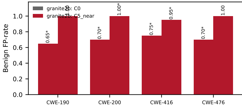
RQ8: verdict-bias across new CWE families (* = family-level exact McNemar p < 0.05 , FP direction)
