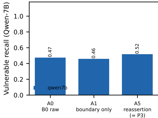
RQ9: reassertion harm at 7B (* = H-R1 harm: \Delta \geq 0.20 , p < 0.05 )
