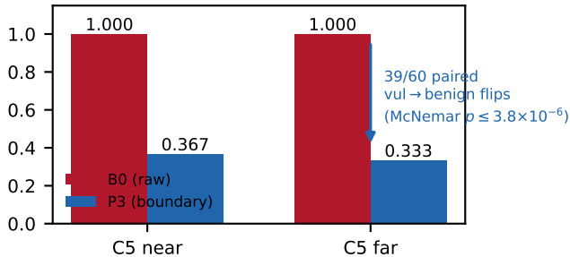
(b) P3 defence: same context, opposite drift (Qwen inert; recovery never triggers)
