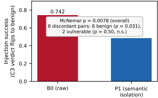
Figure 3: E6: injection success under C3 (share of paired samples whose verdict flips to benign vs. the clean prediction). P1 semantic isolation reduces the aggregate from 0.742 to 0.484 (McNemar p = 0.0078 ), but 6 of the 8 discordant pairs are benign ground truth ( p = 0.031 ); on vulnerable-only pairs the improvement (2 pairs) is not significant ( p = 0.5 ). Source: outputs/experiments/round3_e6/results.json.
