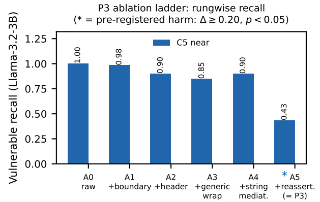
Figure 7: Round 6 (RQ7b): P3 component-ablation ladder (Llama-3.2-3B, C5_near, 60 vulnerable + 30 benign paired functions). Bars: vulnerable recall at each cumulative rung A0 (raw B0) → A1 boundary label only → A2 provenance header → A3 generic comment wrap → A4 string mediation → A5 reassertion (= full P3); the rung that crosses the pre-registered harm threshold ( \Delta \geq 0.20 , McNemar p < 0.05 vs. the previous rung) is marked. Source: outputs/master/round6_ablation.json (frozen decision rules: docs/round6_ablation_prereg.md; execution: configs/round6_ablation.yaml).
