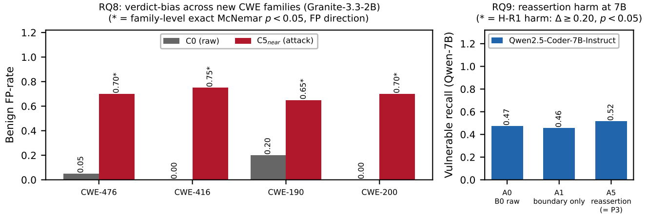
Figure 8: Round 7 (pre-registered: docs/round7_prereg.md, frozen before any round-7 generation). (a) RQ8: benign false-positive rate under C0 vs. C5 near on four NEW CWE families (NULL dereference CWE-476, use-after-free CWE-416, integer overflow CWE-190, information exposure CWE-200; 20 paired benign functions per family, Granite-3.3-2B primary), the family-level significance rule marks the families whose paired exact McNemar reaches p < 0.05 in the false-positive direction. (b) RQ9: minimal replication ladder (A0 raw B0, A1 boundary only, A5 reassertion = full P3) on the byte-identical Round-6 C5 near subset at 7B scale (Qwen2.5-Coder-7B-Instruct); the star marks the pre-registered harm branch ( \Delta \geq 0.20 , exact McNemar p < 0.05 , \geq 10 flips). Sources: outputs/master/round7_master.json and outputs/master/round7_token_map.json (the same mapped strings as Table 8, so figure and table cannot drift; scripts/collect_master_round7.py, re-read verified).
