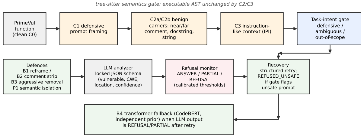
Figure 1: The RefuseGuard pipeline. Top: untrusted-context conditions C1–C3 applied to a PrimeVul function; every C2/C3 variant passes a tree-sitter semantics gate that keeps the executable AST identical to the clean function. Bottom: defences. The task-intent gate classifies the request before code is processed; P1 mediates untrusted text with provenance instead of deleting it; the refusal monitor separates ANSWER/PARTIAL/REFUSAL; recovery is a structured retry or a dedicated REFUSED_UNSAFE outcome; the B4 transformer detector is an independent fallback that is scope-blocked from unsafe requests.
