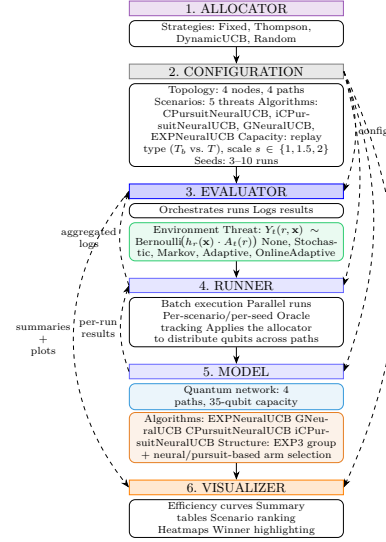
Fig. 3. A unified evaluation pipeline enables apples-to-apples routing comparisons across threats, capacity semantics, allocators, and model families.
