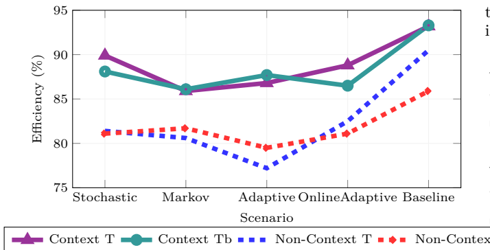
Fig. 9. Contextual (CMAB/iCMAB) models maintain higher Oracle-normalized efficiency than non-context EXP3 baselines across threats under both T and T_b .
