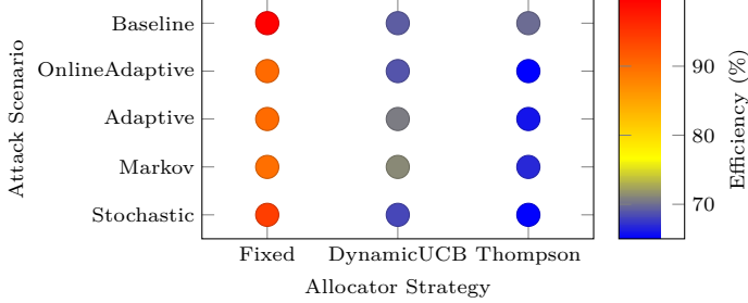
Fig. 6. Efficiency heatmap for CPursuitNeuralUCB across allocator strategies and threat scenarios. In this setting, the Fixed allocator yields the highest efficiency across scenarios, reinforcing allocator choice as a first-class robustness factor.
