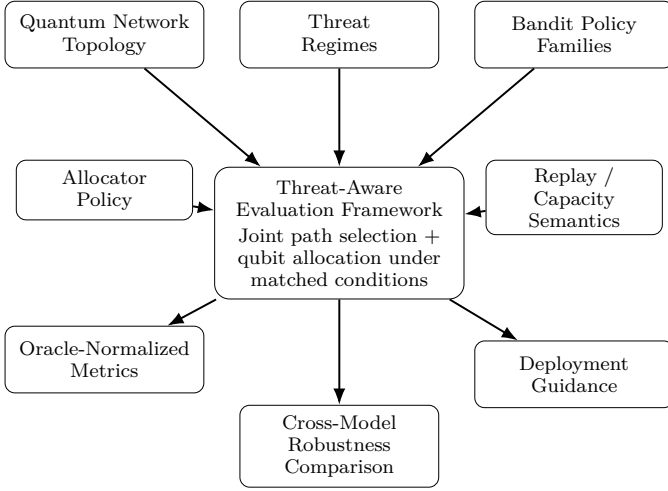
Fig. 1. Threat-aware evaluation framework for quantum entanglement routing. The framework combines network topology, threat regimes, bandit policy families, allocator policy, and replay/capacity semantics under matched conditions to produce Oracle-normalized metrics, cross-model robustness comparisons, and deployment guidance.
