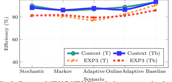
Fig. 2. Contextual (CMAB/iCMAB) methods are more scale-robust than EXP3 baselines, with the clearest Oracle-normalized efficiency gap under T_b settings.
