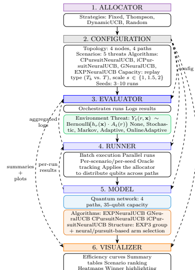
Fig. 1. A unified evaluation pipeline enables apples-to-apples routing comparisons across threats, capacity semantics, allocators, and model families.
