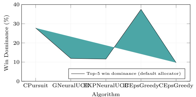
Fig. 6. iEpsilonGreedy wins most often under the default allocator, with CPursuit second.
