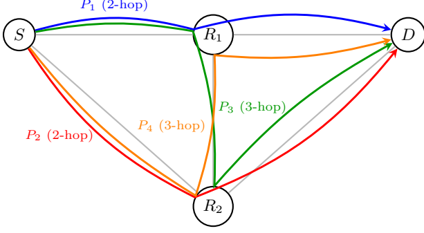
Fig. 5. The testbed exposes four alternative entanglement paths whose qubit splits vary by allocator strategy.
