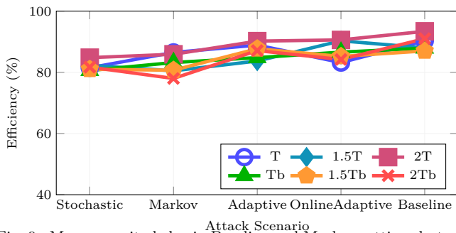
Fig. 9. More capacity helps in Baseline and Markov settings but can hurt under Adaptive threats, revealing the capacity paradox.
