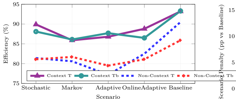
Fig. 7. Contextual (CMAB/iCMAB) models maintain higher Oracle-normalized efficiency than non-context EXP3 baselines across threats under both T and T_b .
