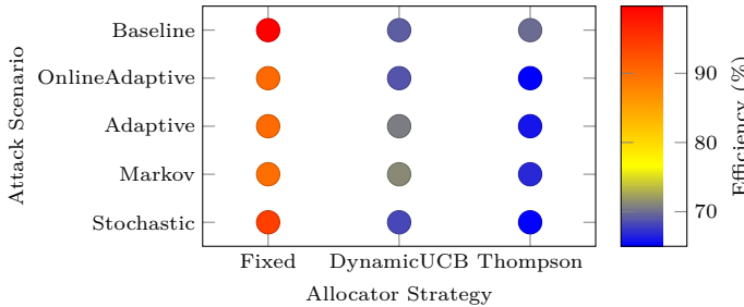
Fig. 4. Efficiency heatmap for CPursuitNeuralUCB across allocator strategies and threat scenarios. In this setting, the Fixed allocator yields the highest efficiency across scenarios, reinforcing allocator choice as a first-class robustness factor.
