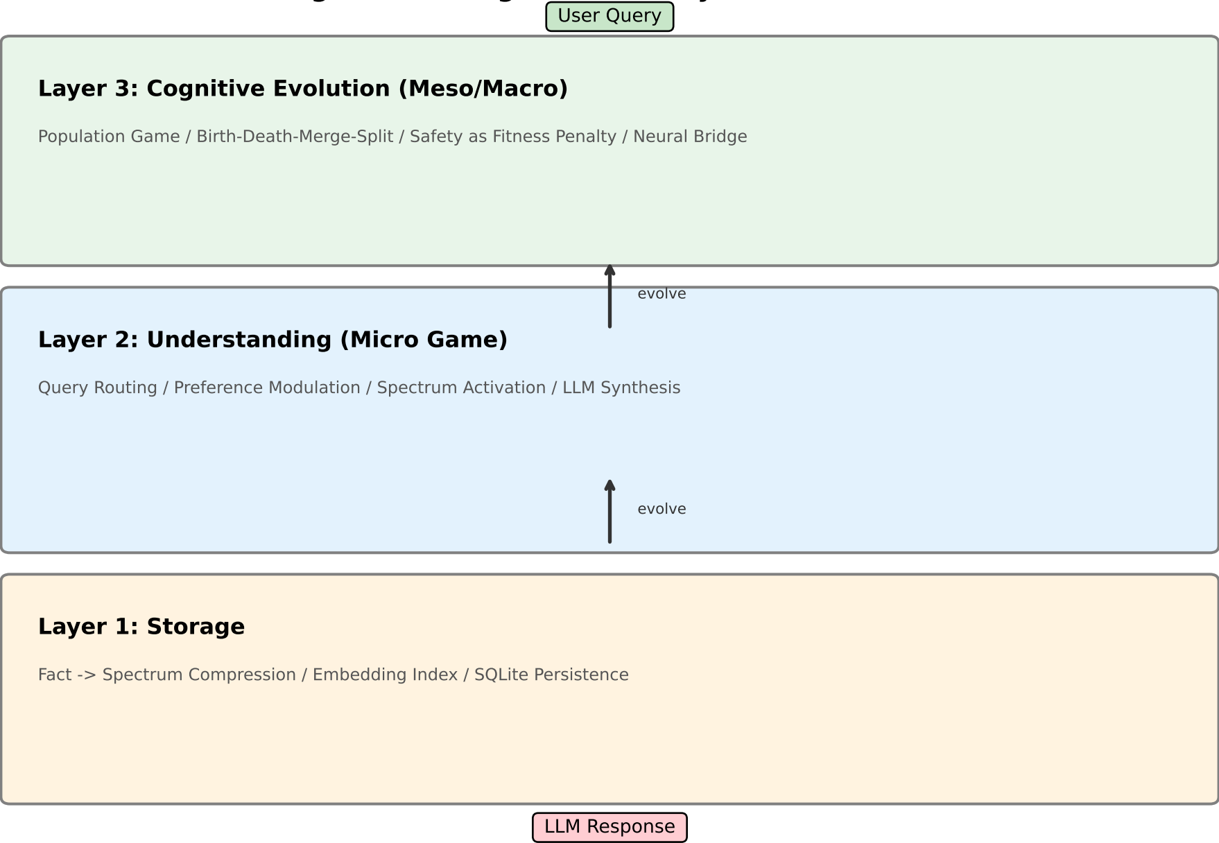
Figure 1: M-Engine Three-Layer Architecture
