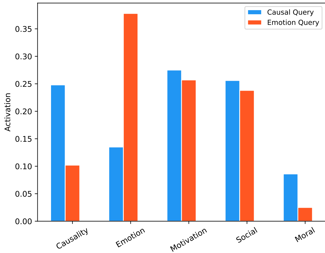
Attention: Same Fact, Different Queries
