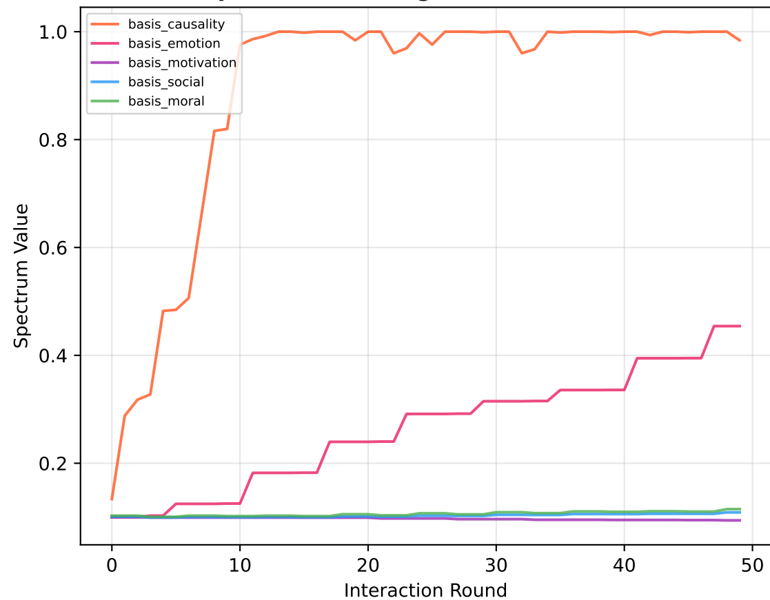
Spectrum Convergence (50 Rounds)
