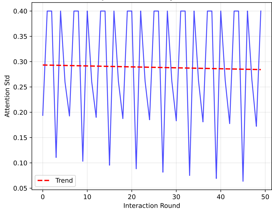
Perspective Diversity Over Time
