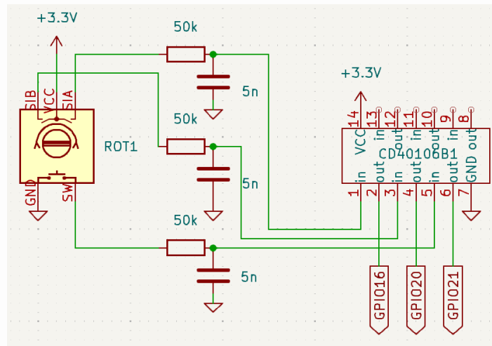
rotary encoder
