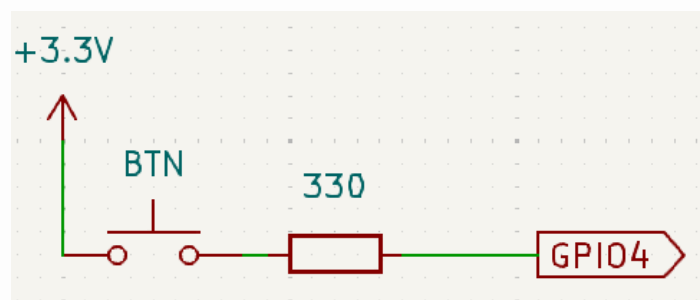
push button circuit
