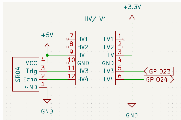
HC-SR04 circuit
