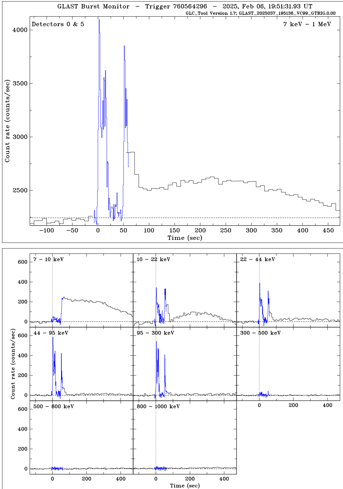
Figure 1: Light curves of the two brightest trigger detectors combined (top); and in the 8 energy channels (bottom).
