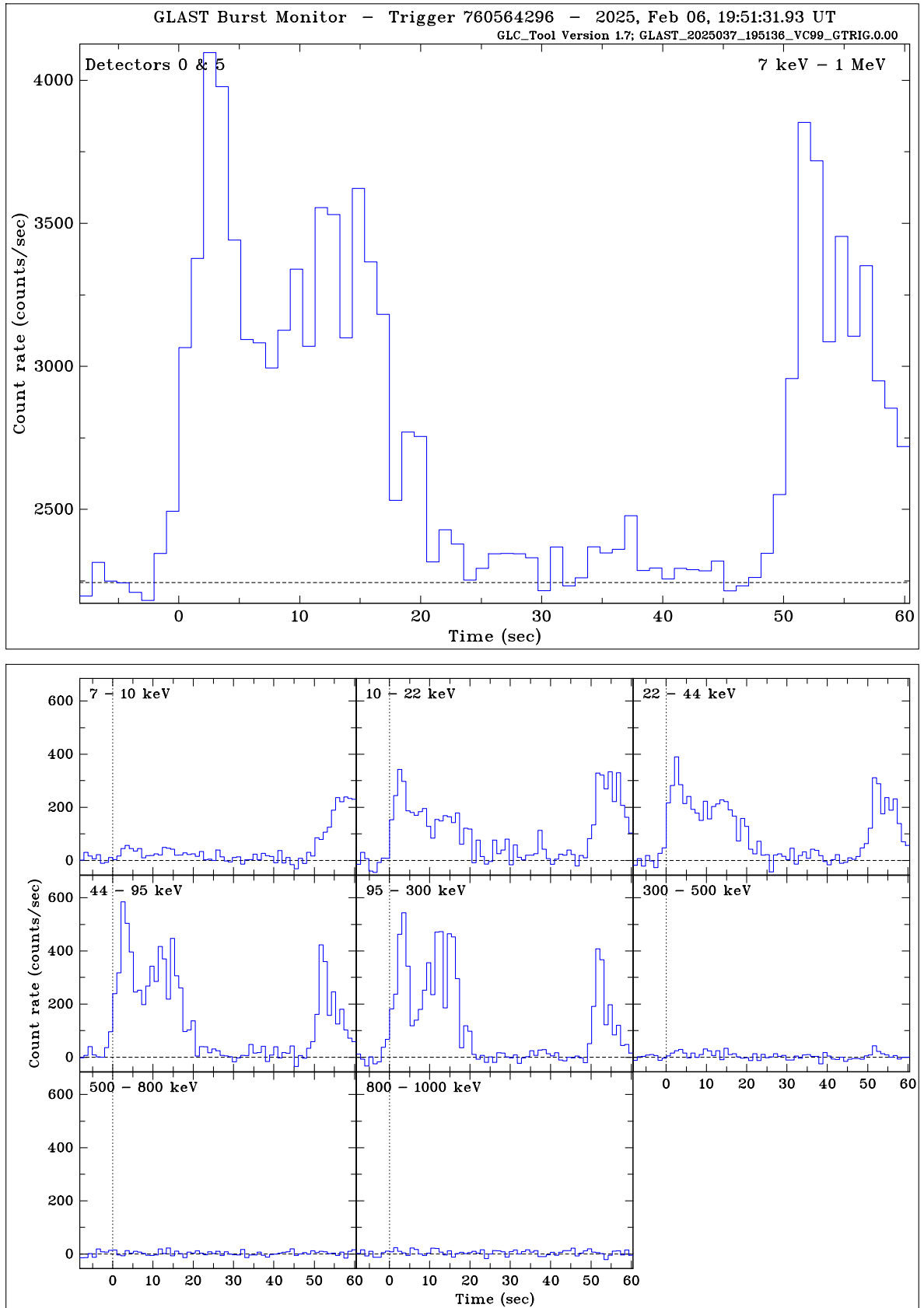
Figure 2: Light curves of the two brightest trigger detectors combined (top); and in the 8 energy channels (bottom).
