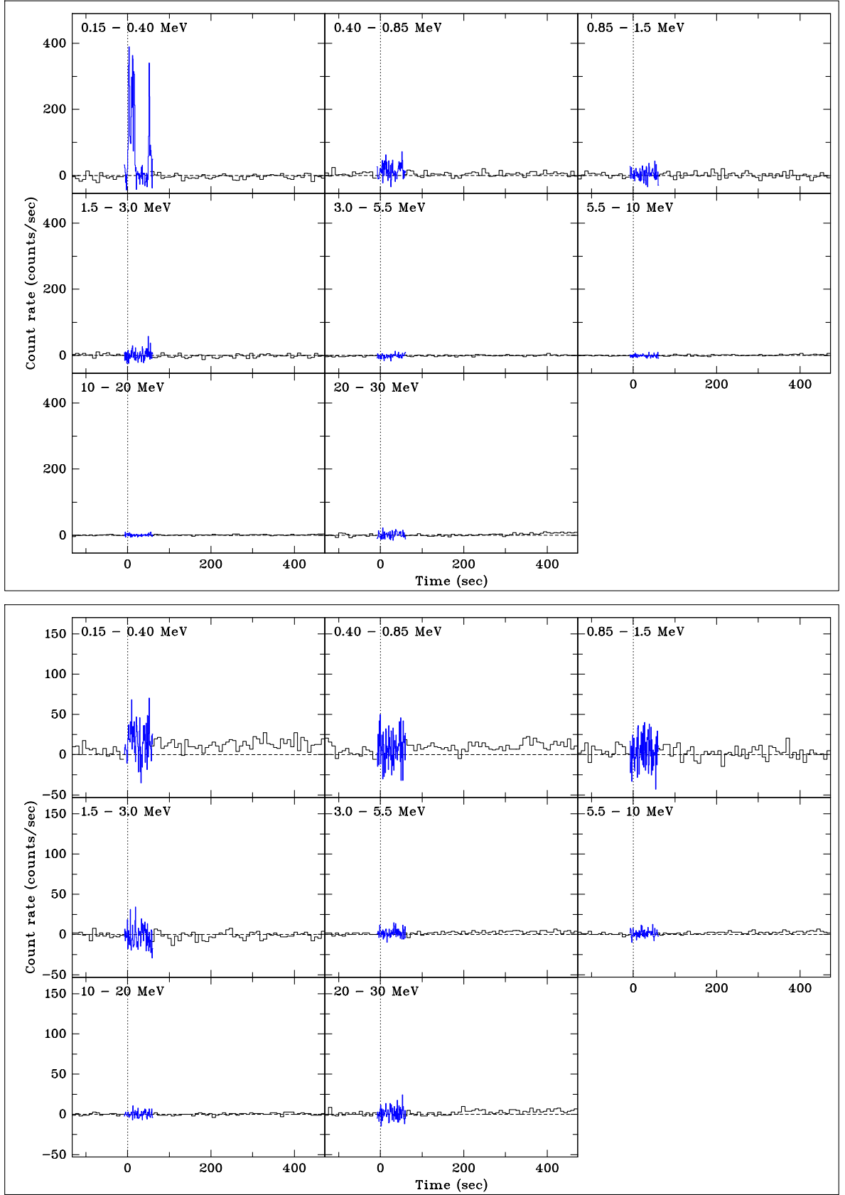
Figure 4: Light curves in 8 energy channels of BGO detector 12 (top) and 13 (bottom).
