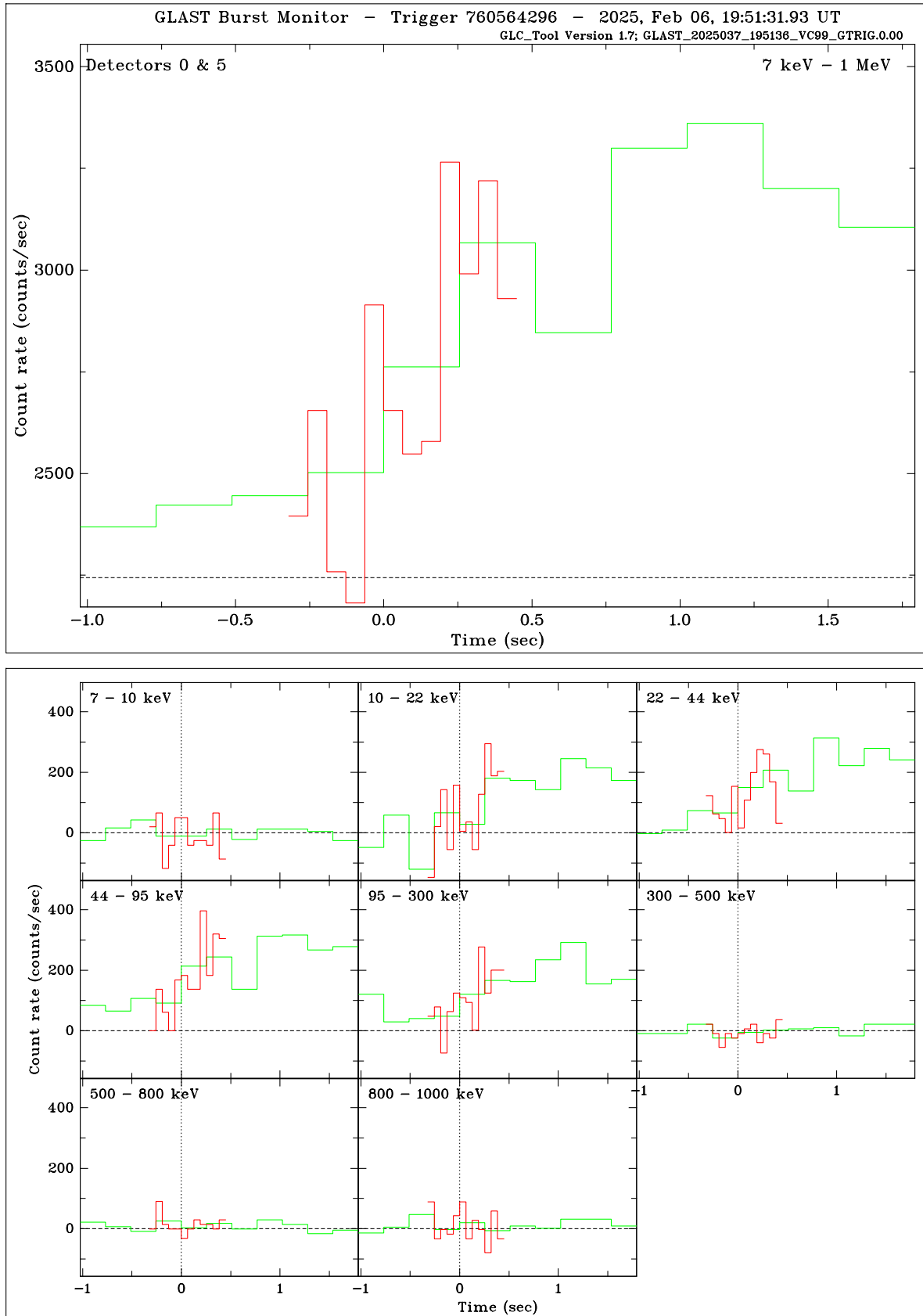
Figure 3: Light curves of the two brightest trigger detectors combined (top); and in the 8 energy channels (bottom).
