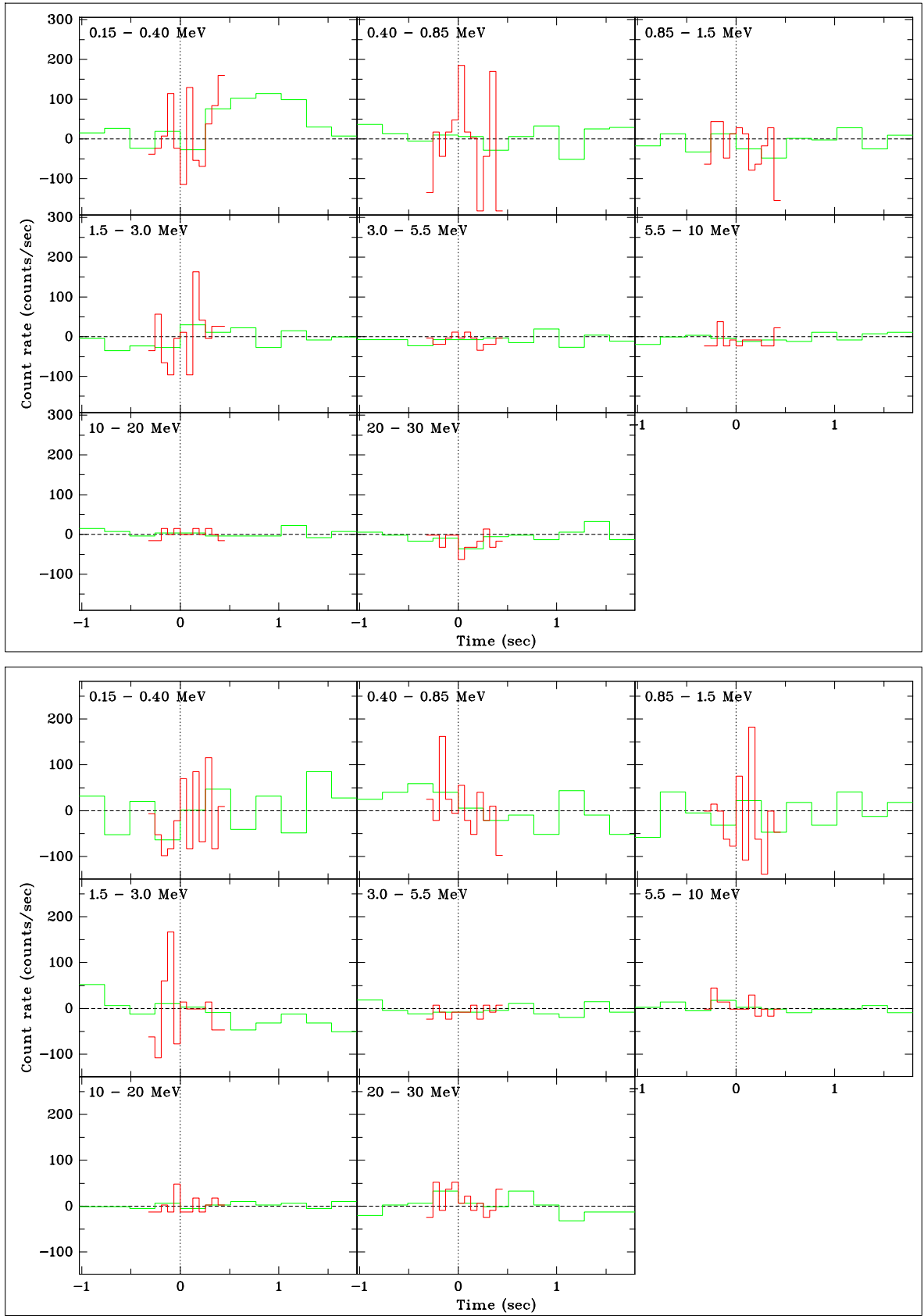
Figure 6: Light curves in 8 energy channels of BGO detector 12 (top) and 13 (bottom).
