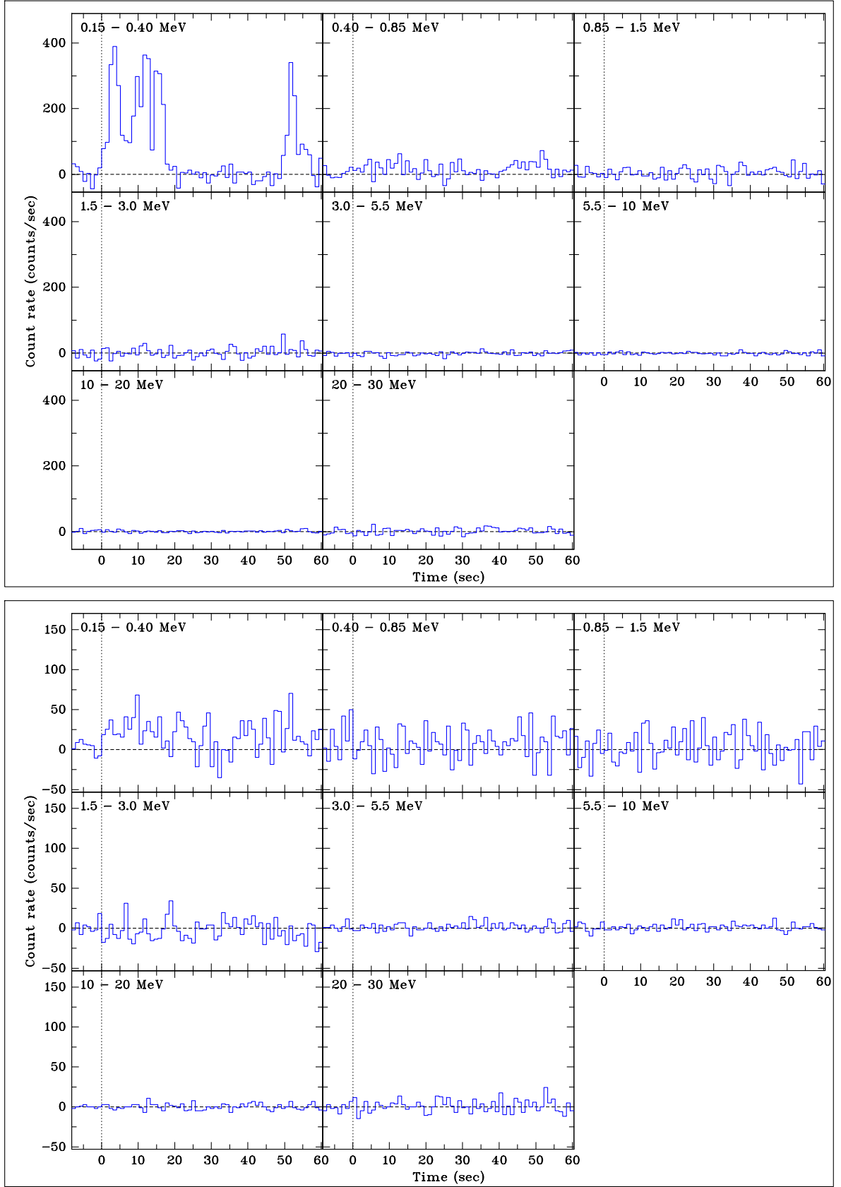
Figure 5: Light curves in 8 energy channels of BGO detector 12 (top) and 13 (bottom).
