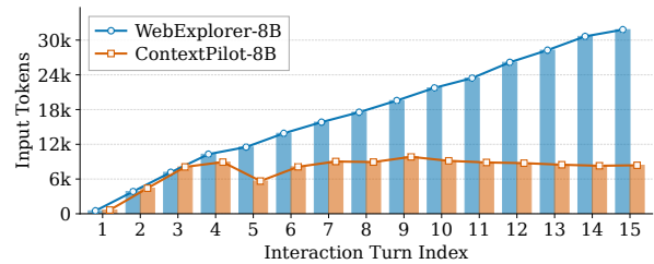
Figure 4. Token usage per turn on BrowseComp.
