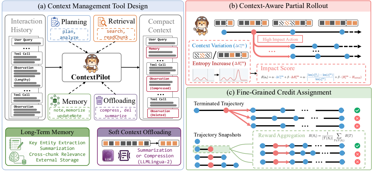
Figure 1. Overview of ContextPilot : (a) Extending the context management tools to support planning, long-term memory, and soft context offloading; (b) Improved RL training algorithm with context-aware partial rollout and (c) fine-grained snapshot-level credit assignment.
