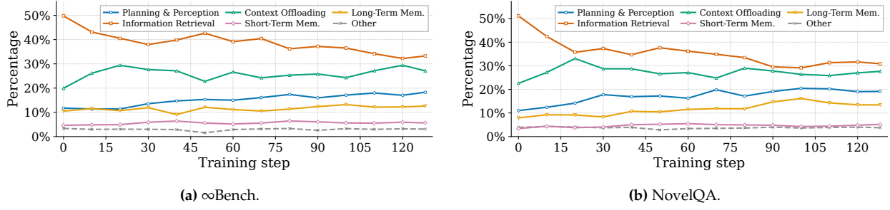
Figure 5. Tool category breakdown during Qwen3-8B RL training on \infty Bench and NovelQA.
