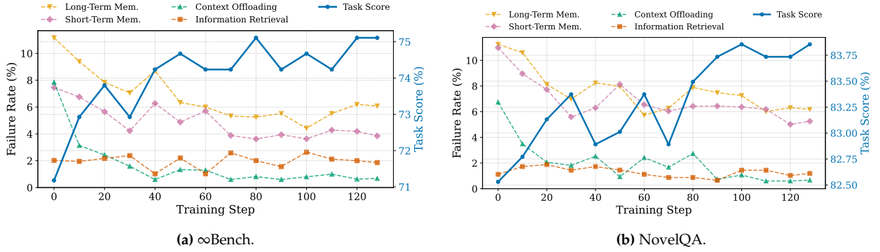
Figure 6. Tool invocation failure rates and task success rate on \infty Bench and NovelQA during RL training.
