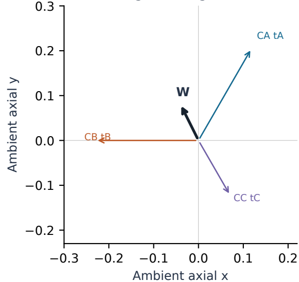
(c) Tangent-weighted sum
